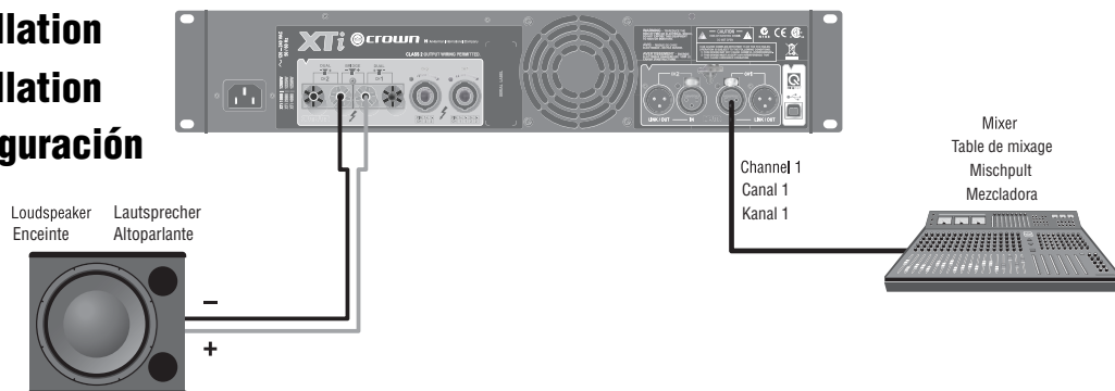
Figure 2.9 Bridge-Mono Wiring of Binding Posts
