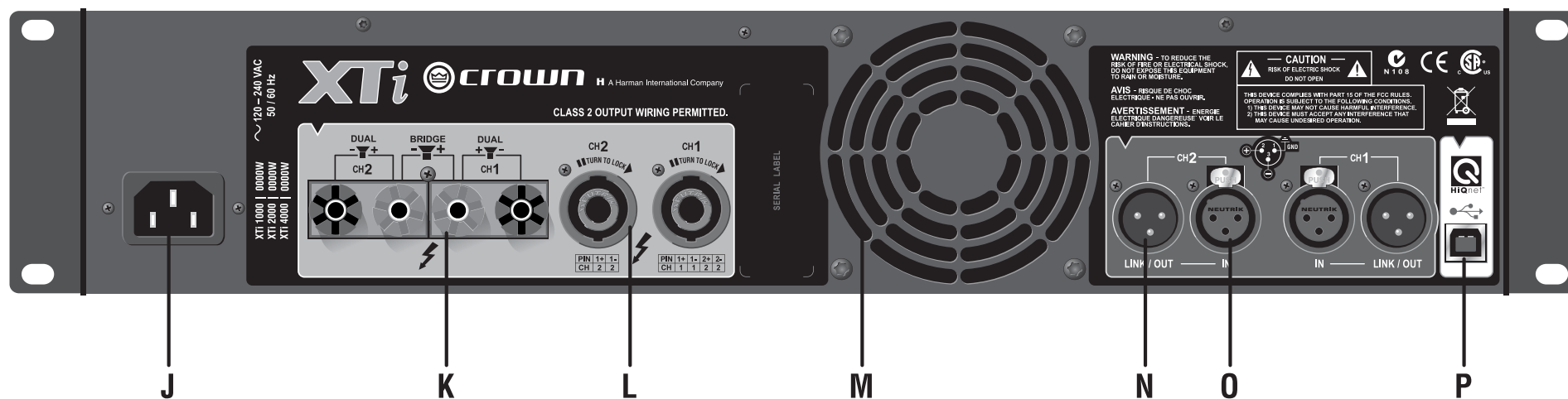
Figure 3.3 Back Panel Controls and Connectors
