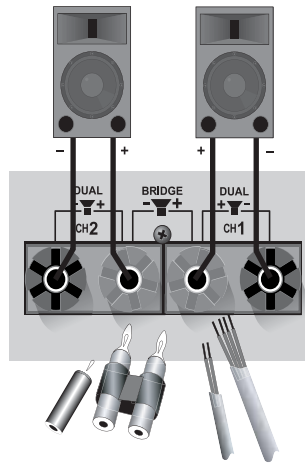
Figure 2.4 Binding Post Output Wiring
