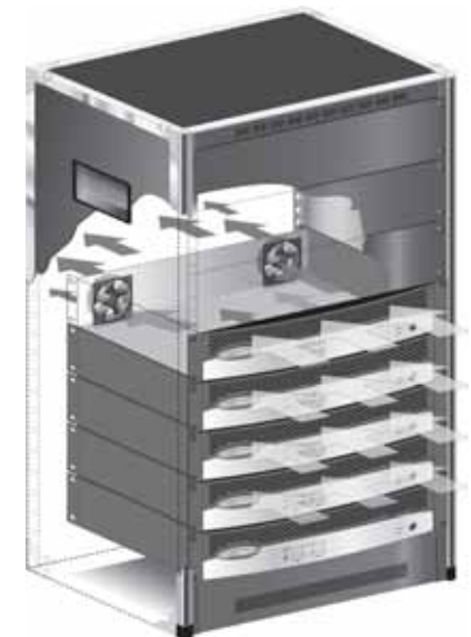
Figure 3.2 Airflow
