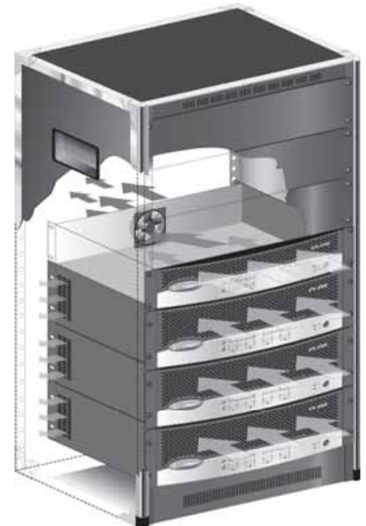
Figure 3.2 Airflow
