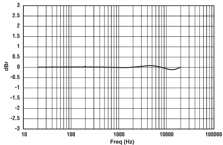
Figure 7.4 CTs 2000/3000 Typical Frequency Response (1W)
