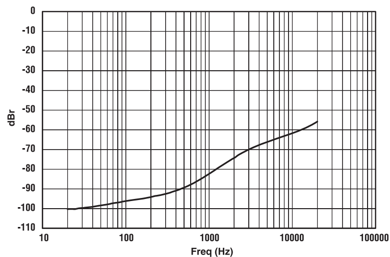
Figure 7.5 CTs 2000/3000 Typical Crosstalk vs. Frequency
