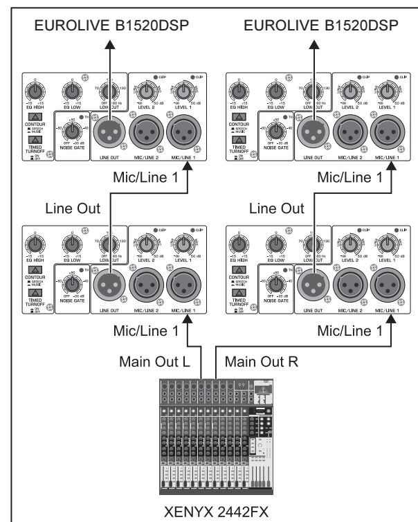
Fig. 4.3: Linking several B1520DSP speakers
