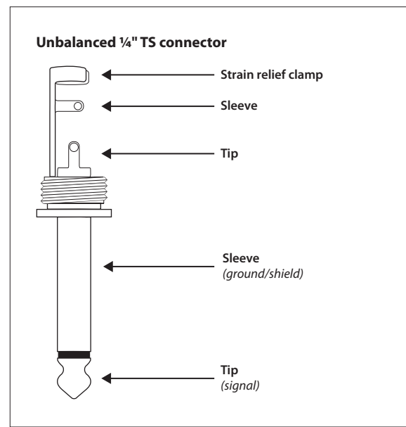
Fig. 5.1: ¼" TS connector
