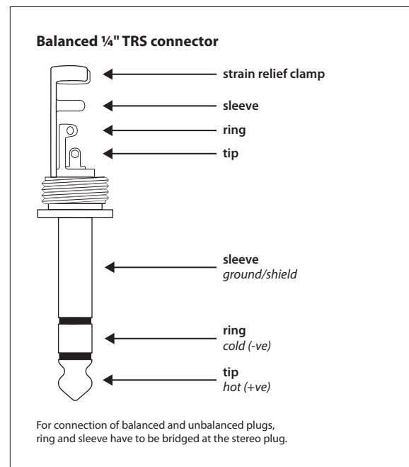
Fig. 5.2: ¼" TRS connector
