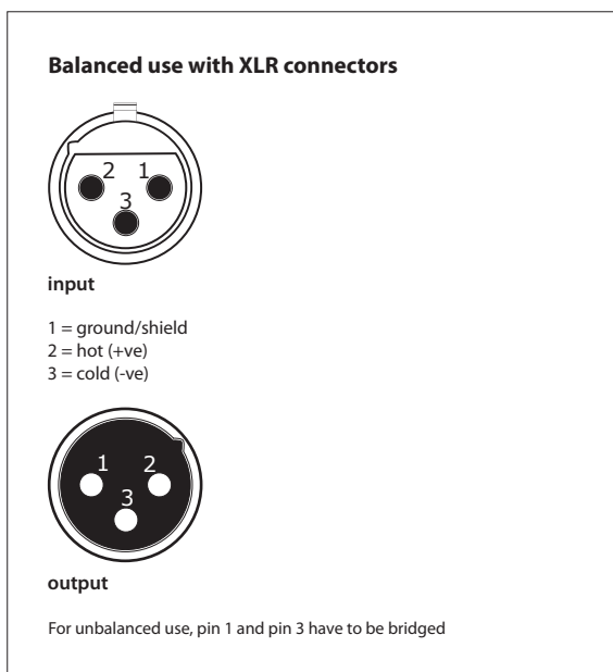
Fig. 5.4: XLR connectors
