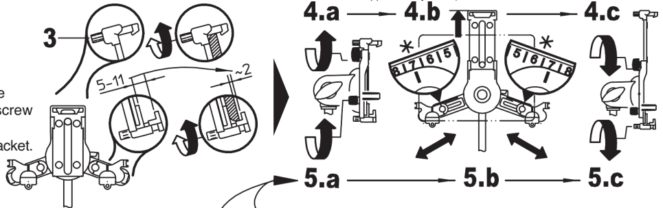
SETUP STAND (1)
