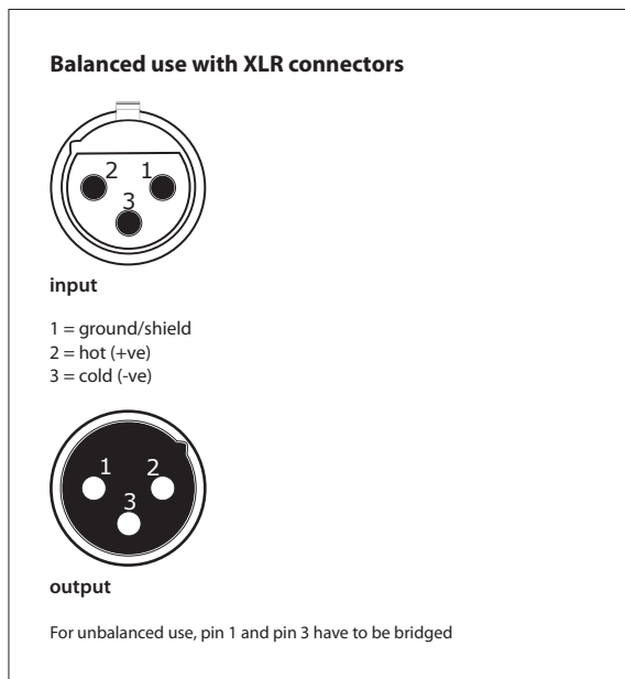
Fig. 3.1: XLR connector
