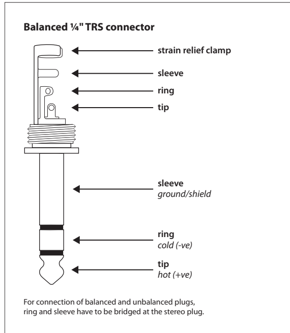
Fig. 3.2: 1/4" TRS connector
