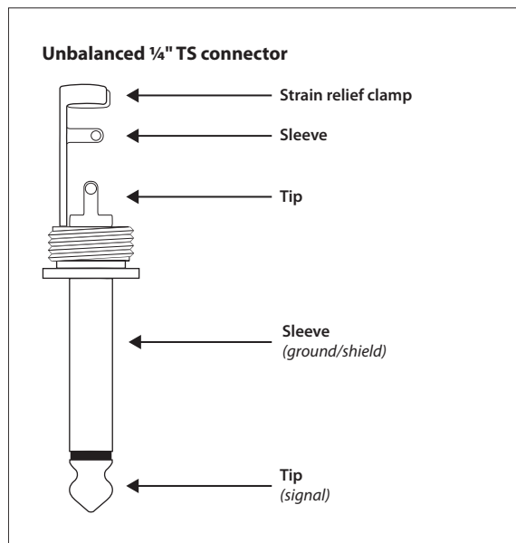
Fig. 3.3: 1/4" TS connector
