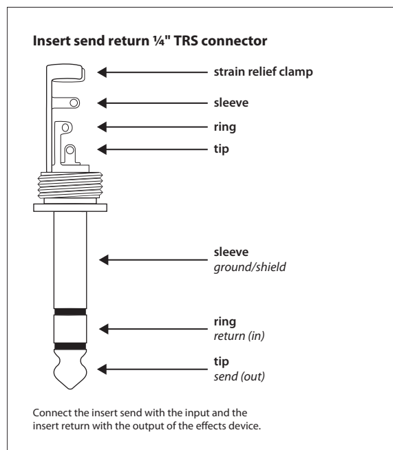
Fig. 3.4: Insert send/return stereo plug
