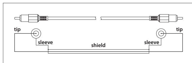
Fig. 3.6: RCA cable
