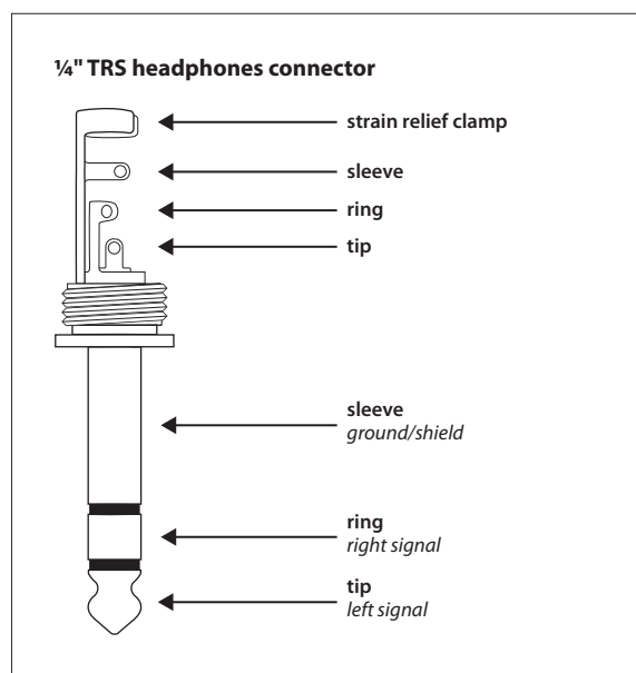
Fig. 3.5: ¼" headphones connector
