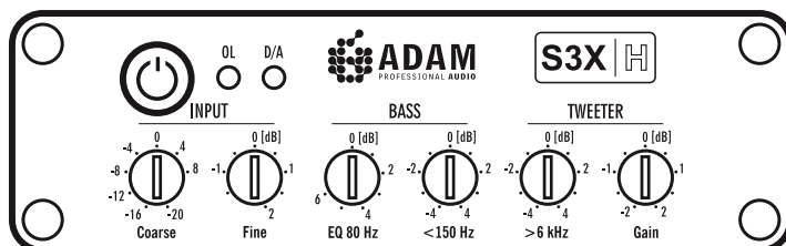
Figure 4: Control panel
