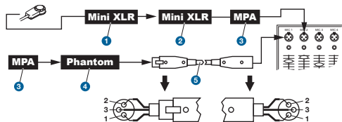
Figure 4: Connection diagram with MPA V L.
