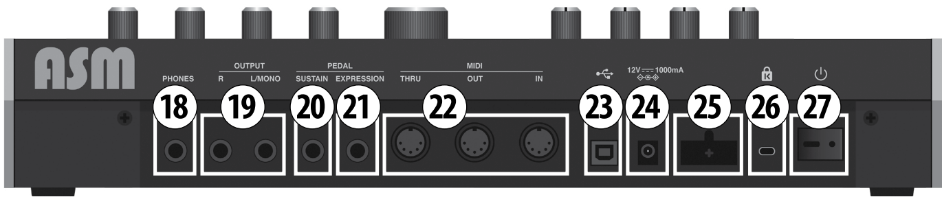
Rear panel of the Hydrasynth desktop model is pictured
