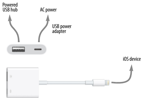
Figure 3-3: The Apple Lightning to USB3 Camera Adapter.
