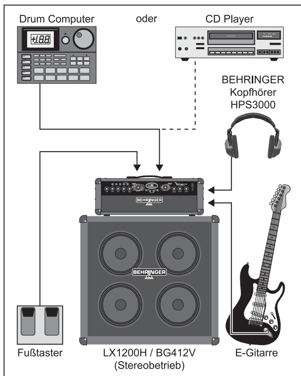
Abb. 3.3: Standard-Setup an 2 x 8 \Omega Impedanz (stereo)
