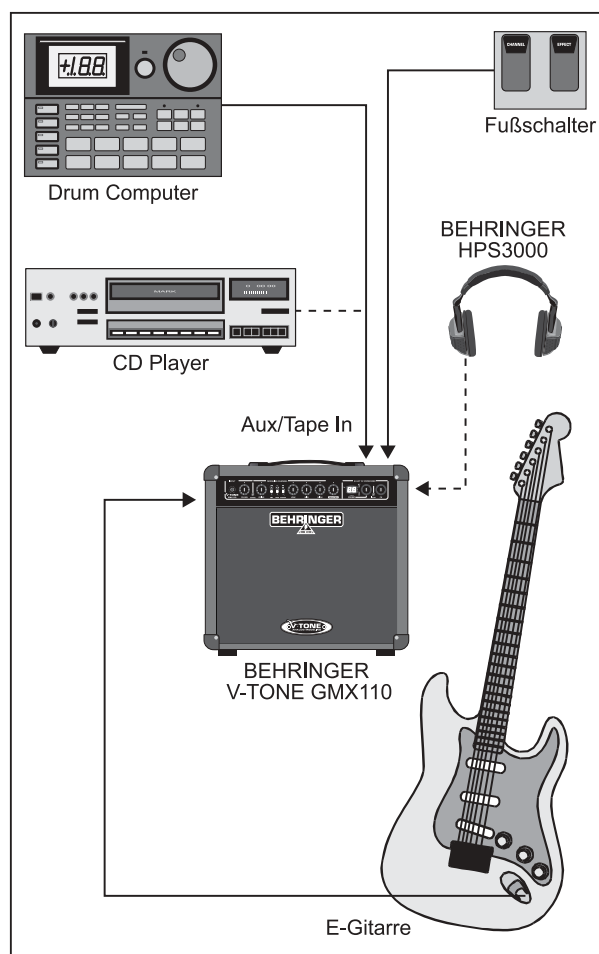
Abb. 3.1: Standard Setup
