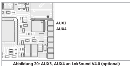
Abbildung 20: AUX3, AUX4 an LokSound V4.0 (optional)
